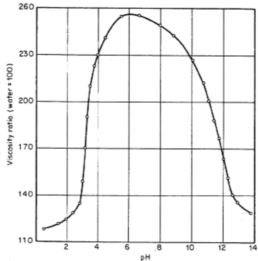
Effect of pH on the viscosity of gum arabic solutions
