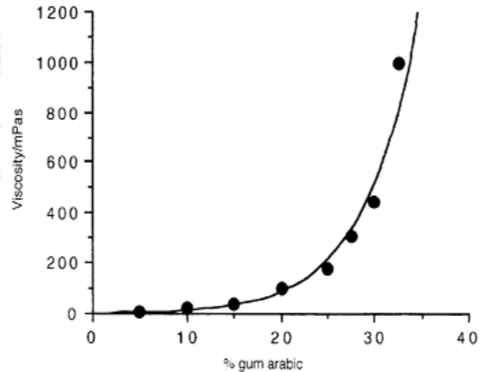
Viscosity of gum arabic as a function of concentration.
